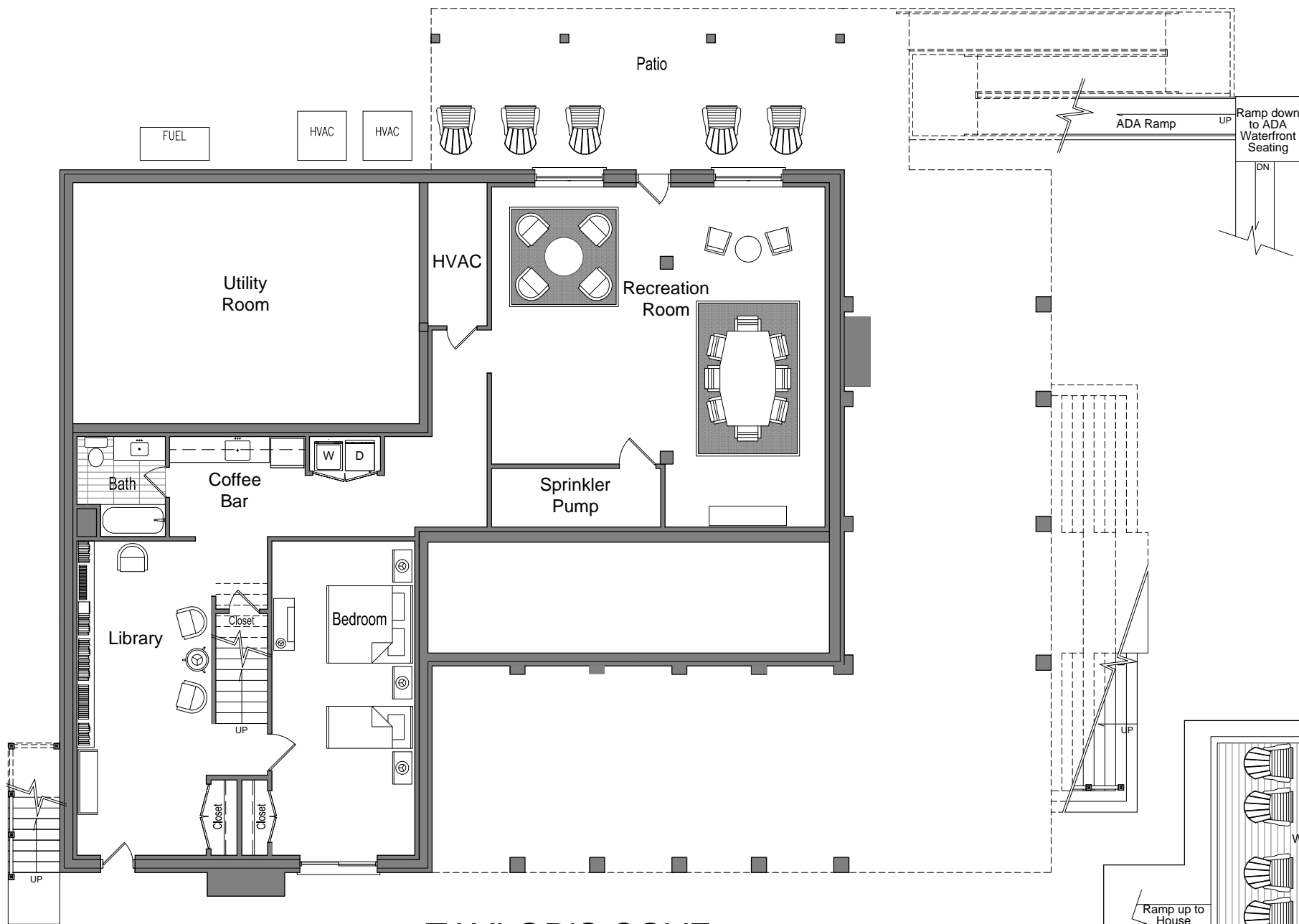
TAYLOR'S COVE LOWER LEVEL PLAN
